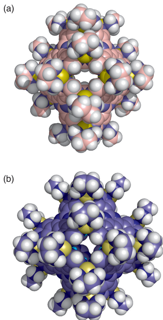
Figure 3. Crystal structures of a) trigonal bipyramidal capsule 1b and b) octahedral capsule 2b ·( 5 ) 4 in space-filling representation (solvents and nitrate ions are omitted for clarity).
